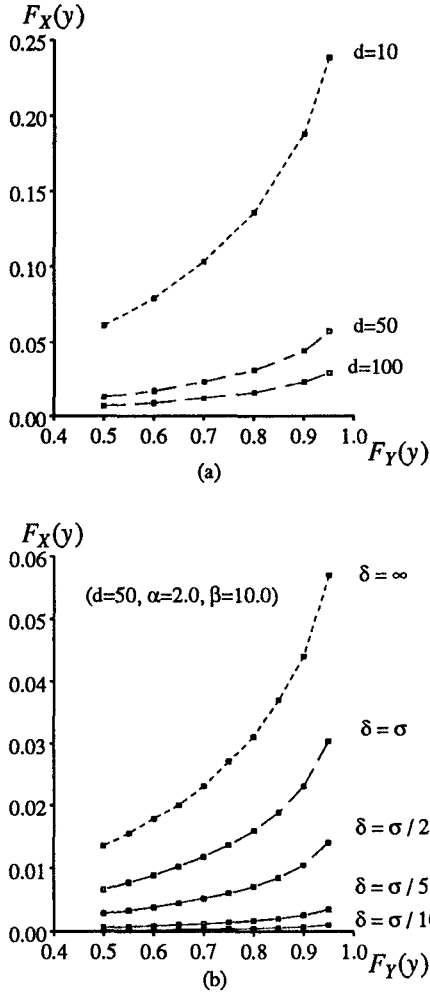
Figure 4.1: The relationship of the strategy cost and local minimum cost distributions: (a) \delta=\infty ; (b) d=50 .
