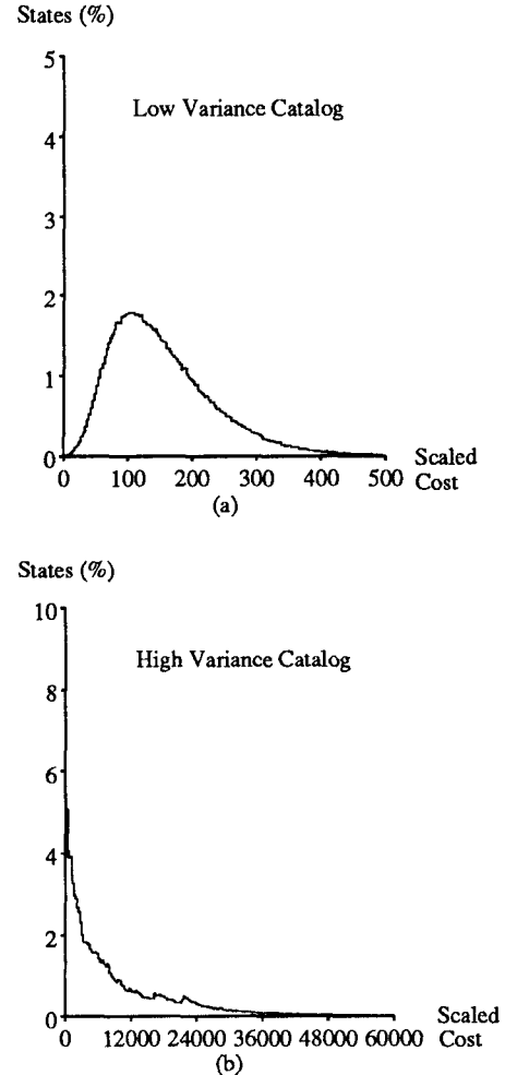
Figure 7.1: The strategy cost distribution of a star query.
